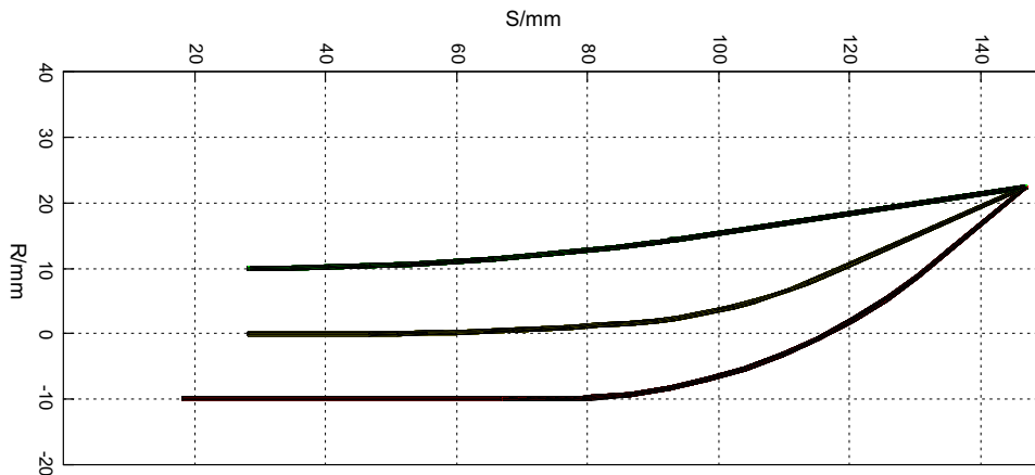
FIGURE 9. Simulation of the remote center of motion like kinematics of the concentric continuum robot. Three needle placement trajectories reach the same target point, achieved by applying different configurations of both the Cartesian base and the concentric tubes.
